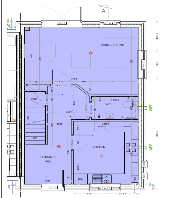
Plot 3 (1 st Flr Plan)
