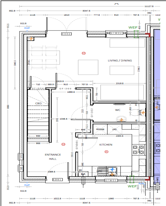
Plots 8, 10, 16 & 18 (Gnd Flr Plan)
