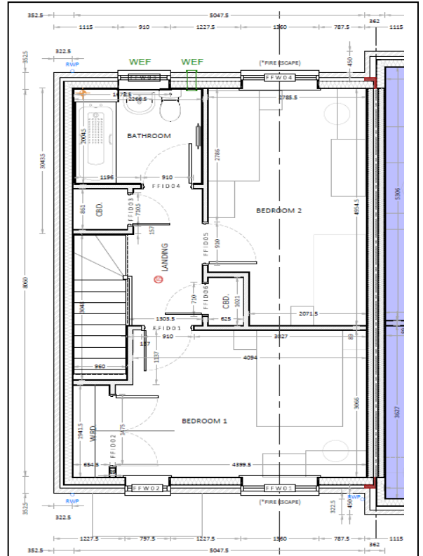
Plots 8, 10, 16 & 18 (1 st Flr Plan)
