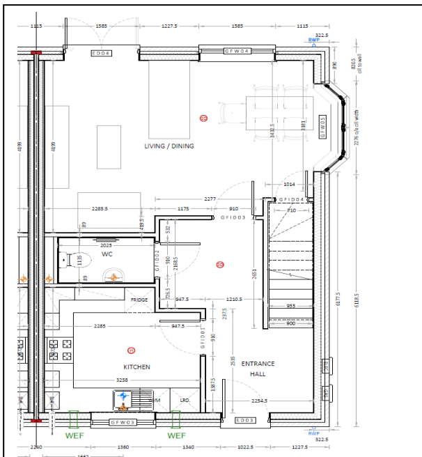
Plots 11 & 20 (Gnd Flr Plan)
