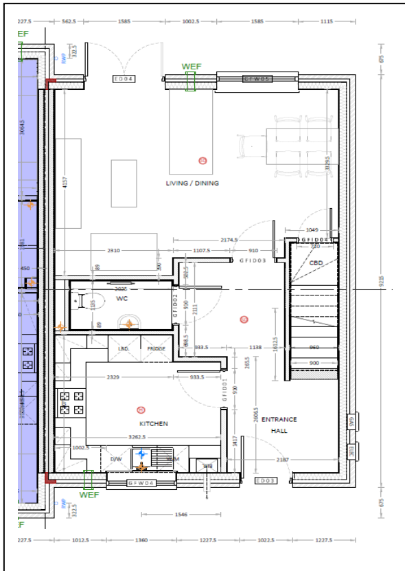
Plot 6 (Gnd Flr Plan)
